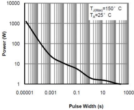
Figure 7: Power Rating
