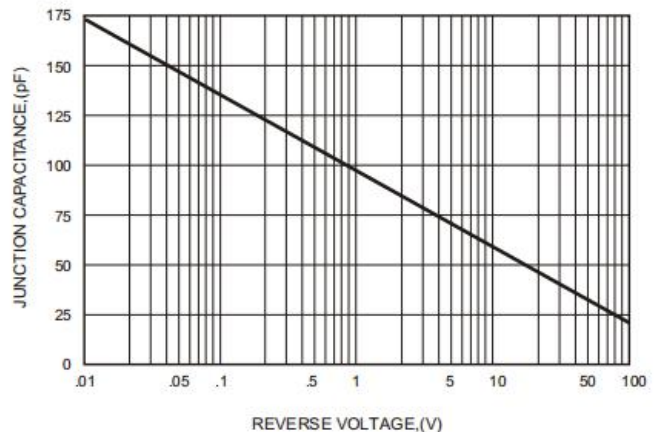
FIG.5-TYPICAL JUNCTION CAPACITANCE
