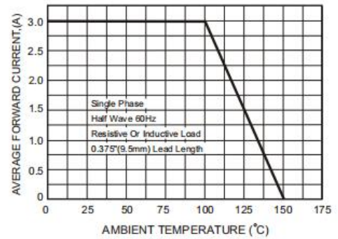
FIG.2-TYPICAL FORWARD DERATING CURVE
