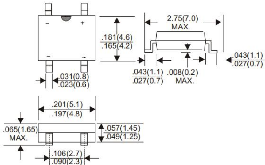
TBS Dimensions in inches and (millimeters)
