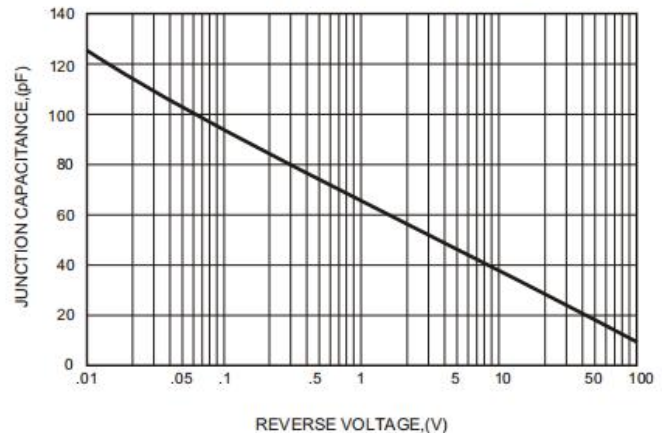
FIG.5-TYPICAL JUNCTION CAPACITANCE
