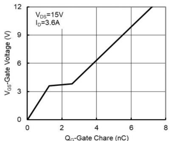
Figure 6: Gate-Charge Characteristics
