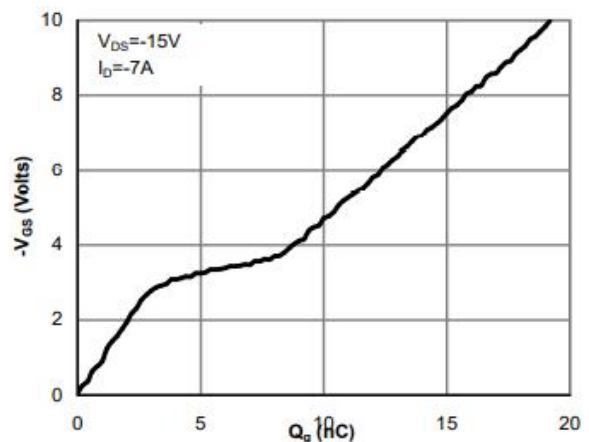
Figure 6: Gate-Charge Characteristics
