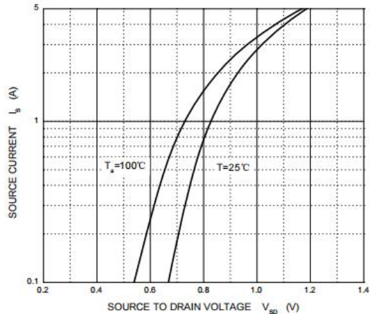
Figure 6: Diode Characteristics
