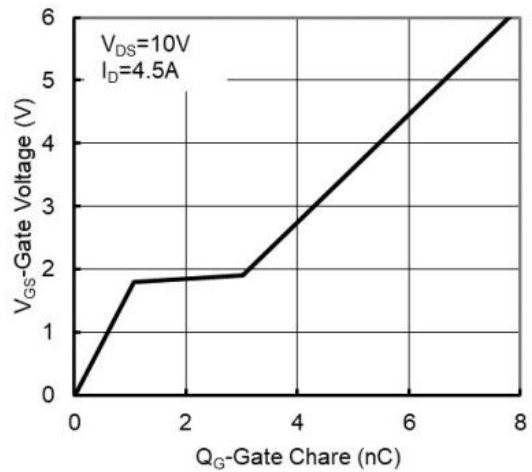
Figure 6: Gate-Charge Characteristics
