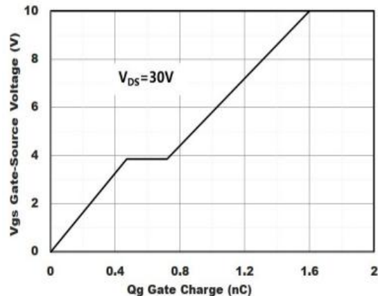
Figure 6: Gate-Charge Characteristics
