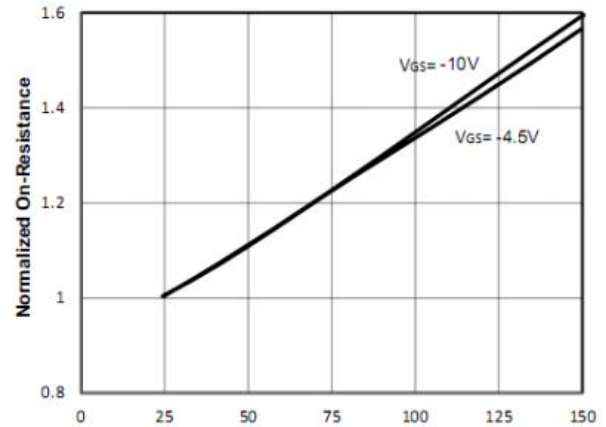
T_J Junction Temperature (°C) Figure 4: On-Resistance vs. Temperature
