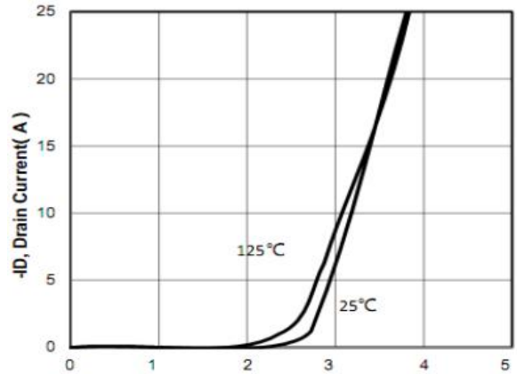
- V_{GS} Gate-Source Voltage (V) Figure 2: Transfer Characteristics
