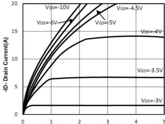
- V_{DS} Drain-Source Voltage (V) Figure 1: Output Characteristics
