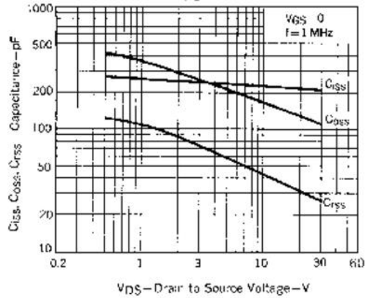
Figure 4: Capacitance Characteristics
