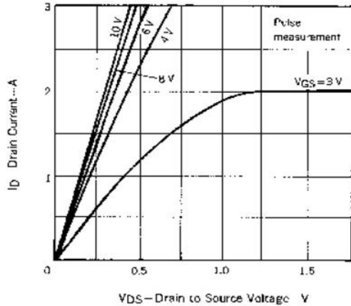
Figure 1: Output Characteristics
